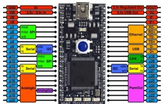
Fig. 3: Pin configuration of embed LPC1768
