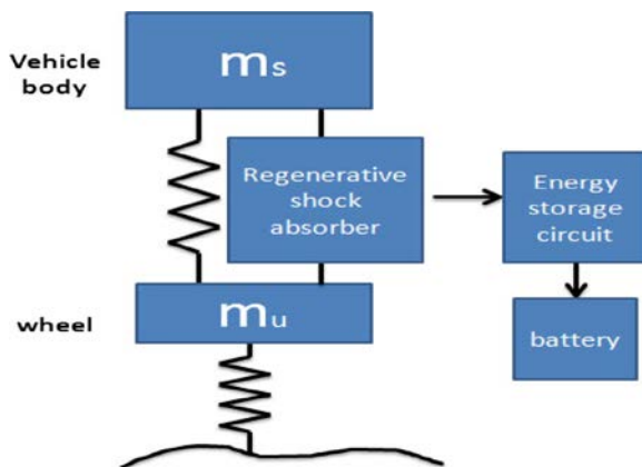
Fig. 4: Typical EM Suspension Model
